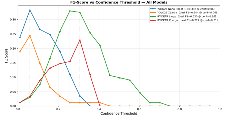
Fig. 6. Confidence Threshold for YOLO26 and RT-DETR models vs F1-Score. The graph shows the optimum confidence level (threshold) in order to maximize the F1 score for each architecture.
